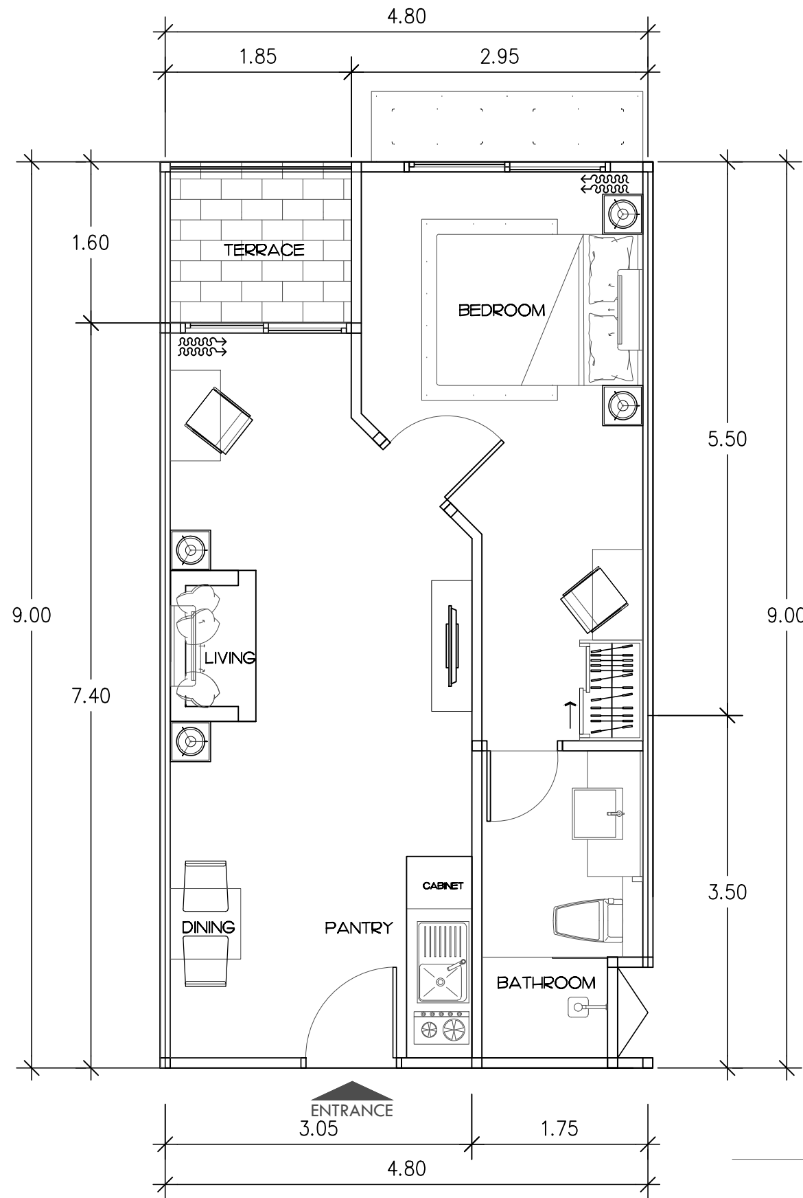
Type A 4 Unit Plan
